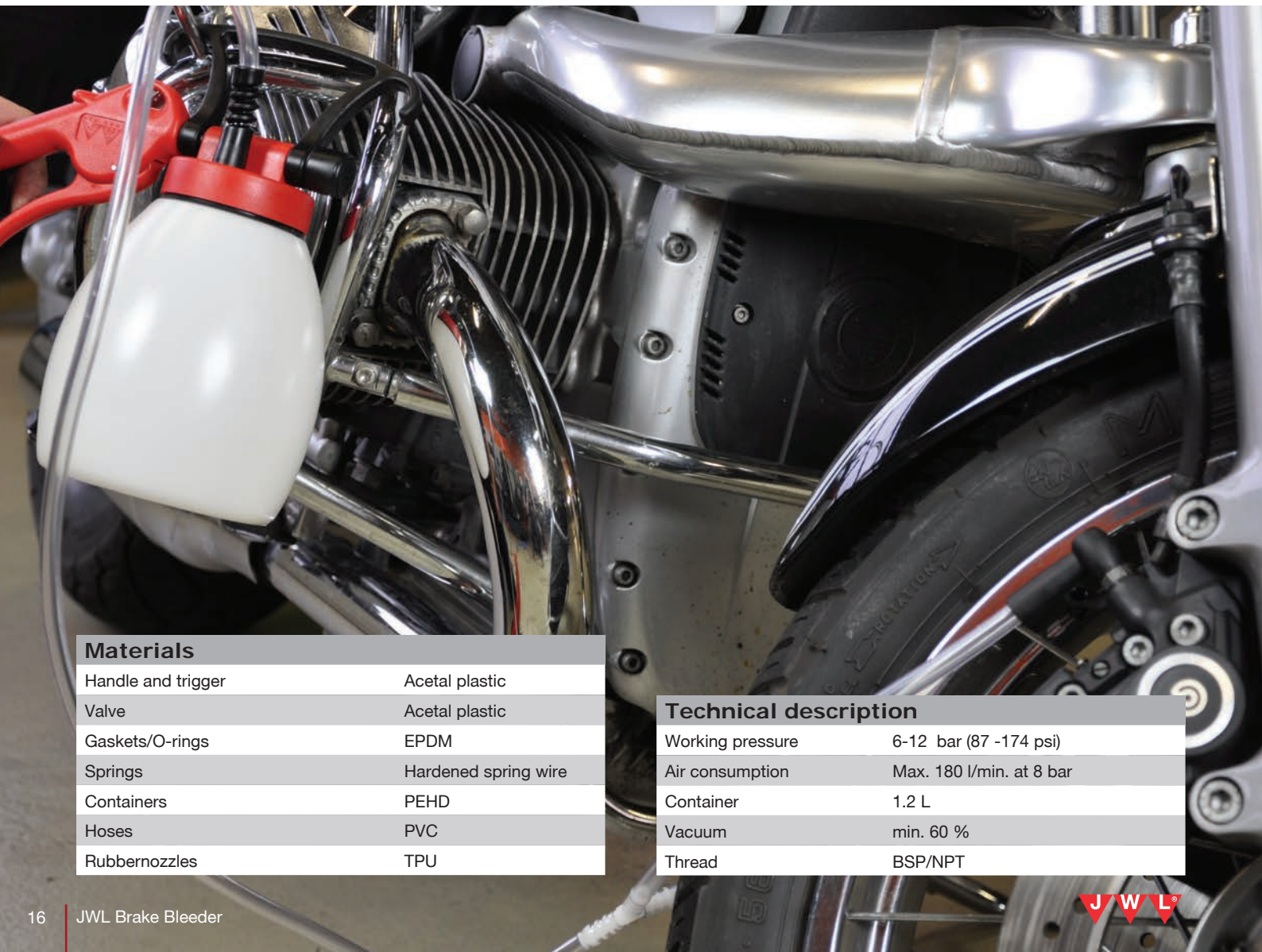
JWL Brake Bleeder is easy to use for one person. Comes with or without replenishment system. Can also be used for MC.
